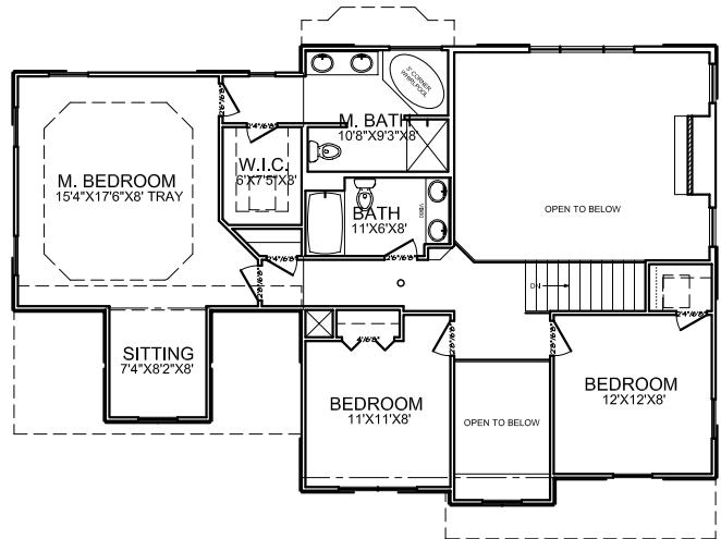
1 SECOND FLOOR PLAN A-5
